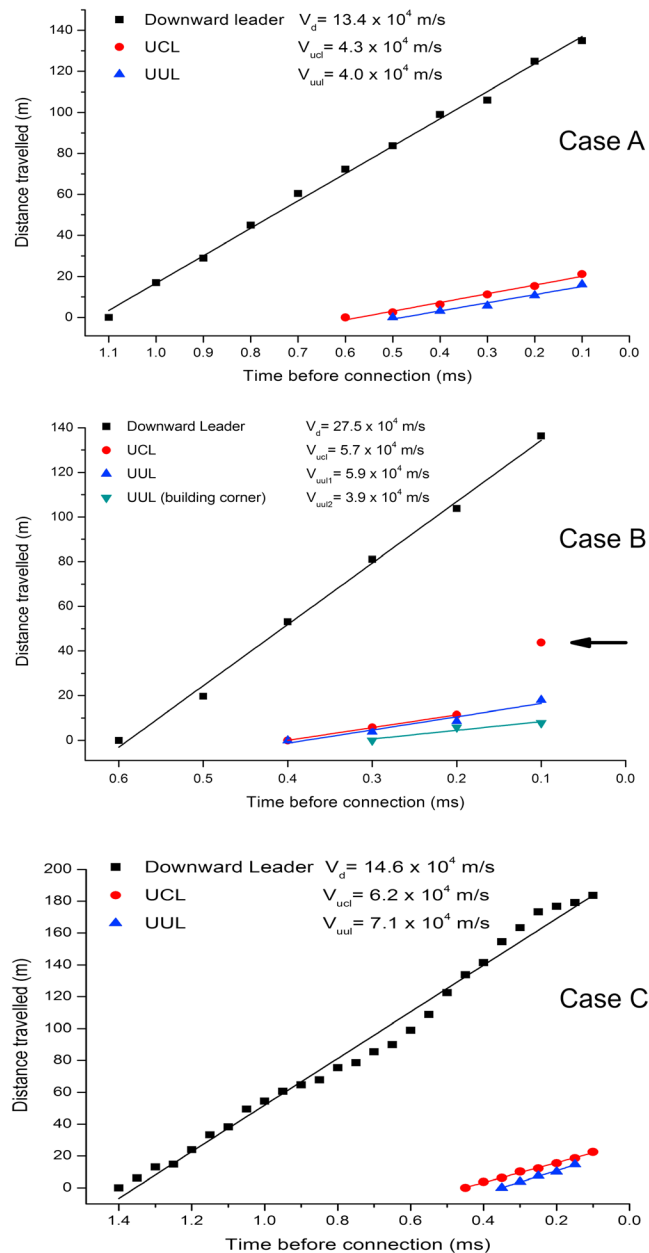
Figure 3. Distance versus time plots and linear regression fits for each case. Each plot starts when the leader first appears in the video image. The average speed for the linear fits are also shown. The connection instant has an uncertainty of frame duration (50 to 100 \mu s).
