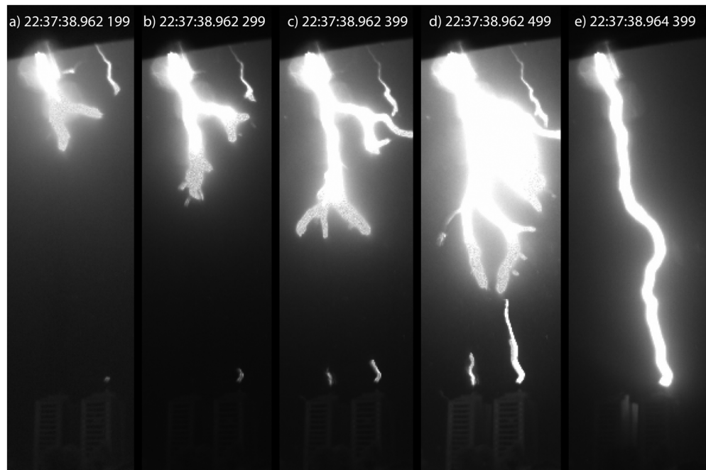
Figure 2. Sequence of video images showing the initiation and development of an UCL on P2 (right-hand side) and two UUL on P1 (left-hand side), one of them being launched from the building corner. This flash (case B) occurred on 1 March 2014. The UT time of each video frame (stamped at the end of the frame integration) is given as hh:mm:ss.xxx yyy (xxx digits are milliseconds and yyy are microseconds).
